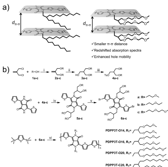
Scheme 1. a) Illustration of the effect of branched OEG side chains. b) Chemical structures and synthetic routes of PDPP3T-O14, PDPP3T-O16, PDPP3T-O20, and PDPP3T-C20. (Reagents and conditions: i) NaH, THF, 0 °C and then 65 °C; ii) \text{BH}_3/\text{THF} , NaOH (aq), \text{H}_2\text{O}_2 (aq), r.t.; iii) (\text{CH}_3)_3\text{N}\cdot\text{HCl} , 4-toluene sulfonyl chloride, \text{Et}_3\text{N} , r.t.; iv) \text{K}_2\text{CO}_3 , (\text{C}_4\text{H}_9)_4\text{NBr} , dimethylformamide, 120 °C; v) N -bromosuccinimide, dichloromethane, r.t.; vi) \text{Pd}_2(\text{dba})_3 , \text{P}(\text{o-tolyl})_3 , chlorobenzene/DMF (10:1, \nu/\nu ), 135 °C).
