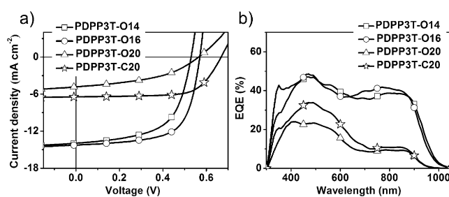
Figure 2. a) J – V and b) EQE curves of the PSC devices based on the four polymers with the active layer thickness of ca. 100 nm.
